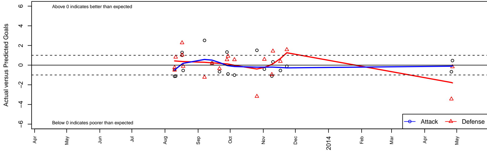
Real So Cal White B99 Dots are actual minus expected GF (blue circles) and GA (red triangles). Blue line is smoothed change in attack strength. Red is smoothed change in defense strength.
